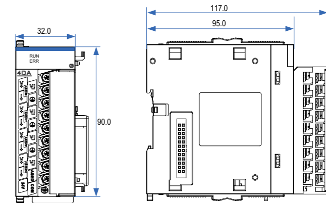
Figure 3 Mounting dimensions diagram (in mm)
